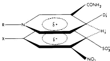
Figure 1. Activated complex for nonlinear hydride transfer.
